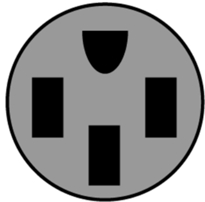
Nema 14-50R (Cooper)
