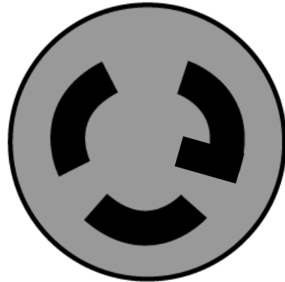
Nema L5-30 (Hartlock)
